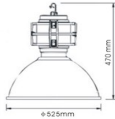
Fixture Sizes (Unit:mm)
